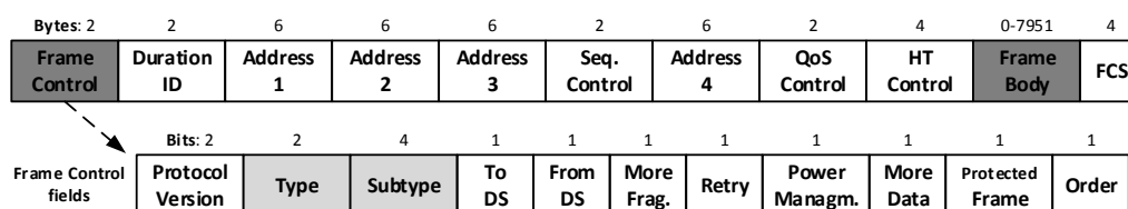
Figure 4.3: IEEE 802.11 MAC frame format (as in IEEE 802.11-2012 standard).
