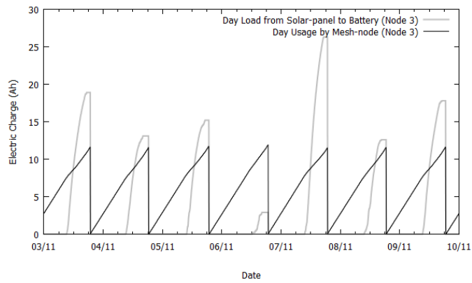
Fig. 12. Battery day load (Ah) along with the mesh node day usage (Ah). Measurements were taken at the mesh node 3 from our real-world wireless mesh network, for a period of one week in winter.
