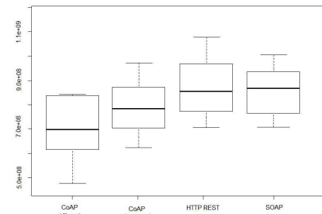
Fig. 9. Service access times (in ns, per protocol)
