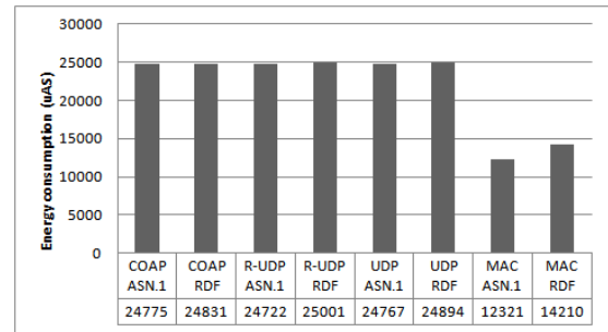
Fig. 8. Energy consumption (in \mu AS, 10min)
