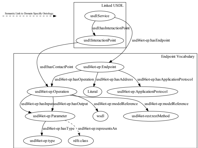
Fig. 4. LUSDL extended by an endpoint vocabulary [14]
